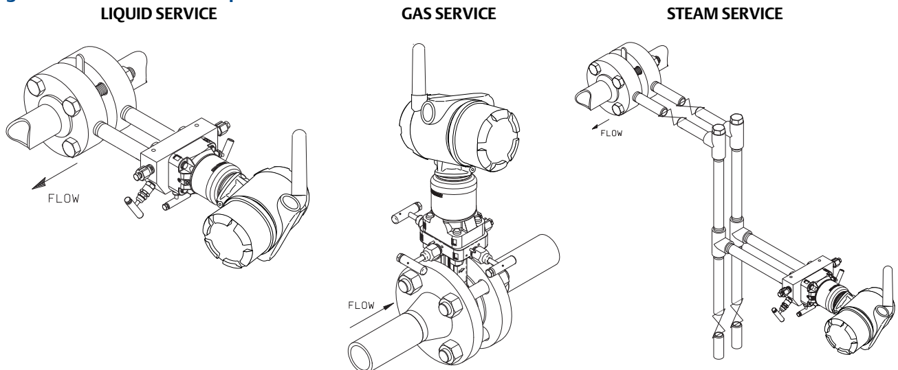
Figure 3-5. Installation Examples
