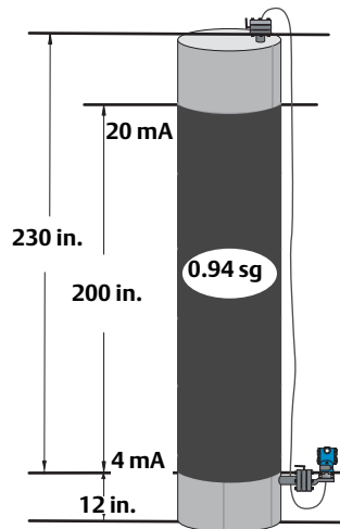
Figure 2-3. Example tank
